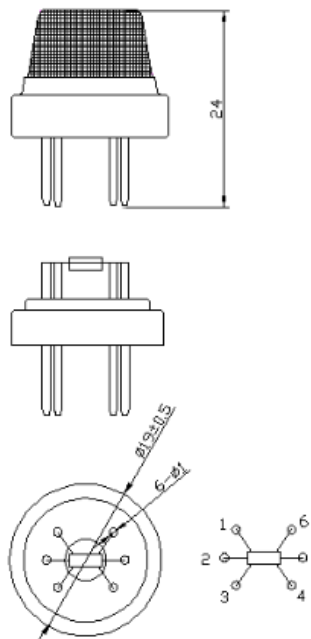
Fig1. Sensor Structure
