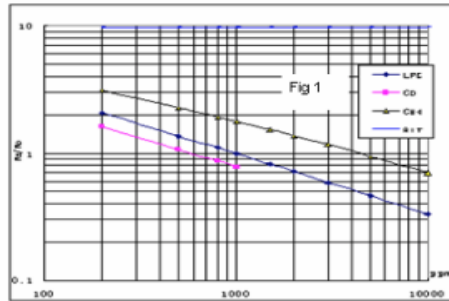
Fig.1 shows the typical sensitivity characteristics of the MQ-9, ordinate means resistance ratio of the sensor ( R_s/R_o ), abscissa is concentration of gases. R_s means resistance in different gases, R_o means resistance of sensor in 1000ppm LPG. All test are under standard test conditions.
