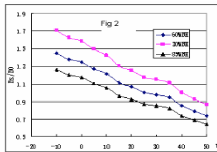
Fig.2 shows the typical temperature and humidity characteristics. Ordinate means resistance ratio of the sensor ( R_s/R_o ), R_s means resistance of sensor in 1000ppm Propane under different tem. and humidity. R_o means resistance of the sensor in environment of 1000ppm Propane, 20°C/65%RH
